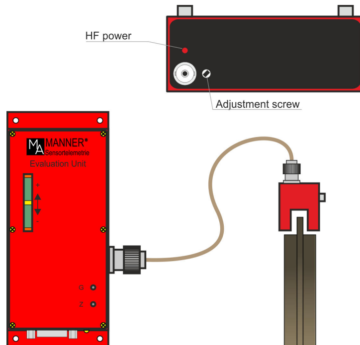
Fig. 7: Stator antenna adjustment
