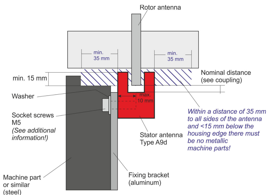
Fig. 6: Minimum distance antenna A9d
