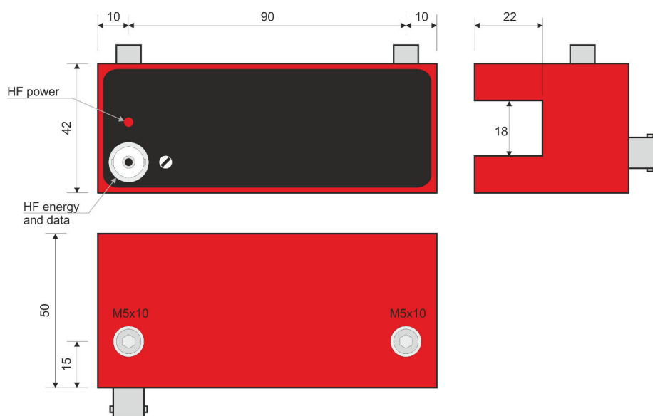
Fig. 4: Stator antenna A9d_PCM
