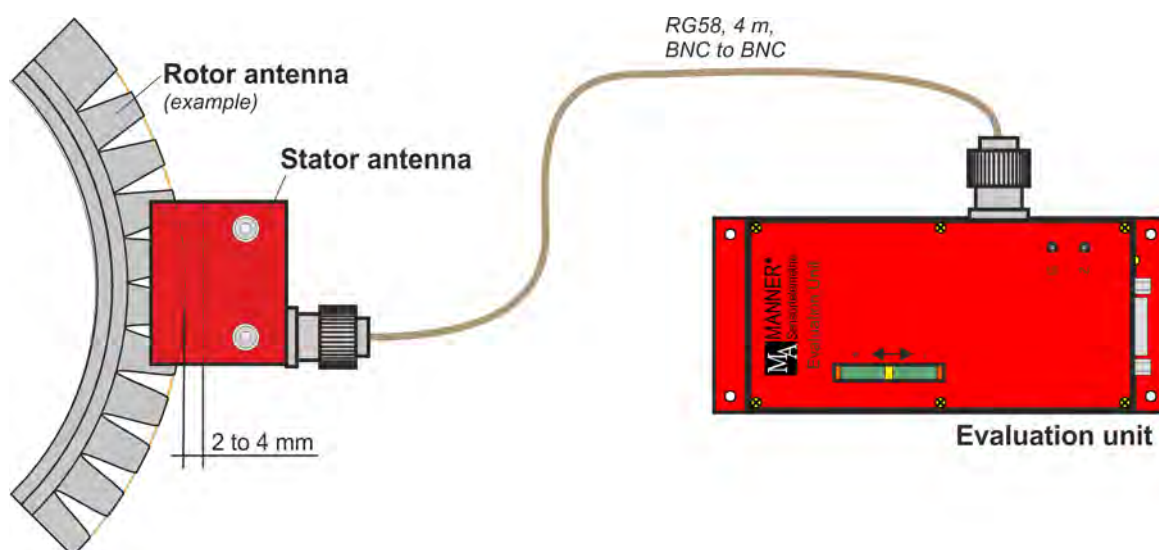
Fig. 5: Coupling
