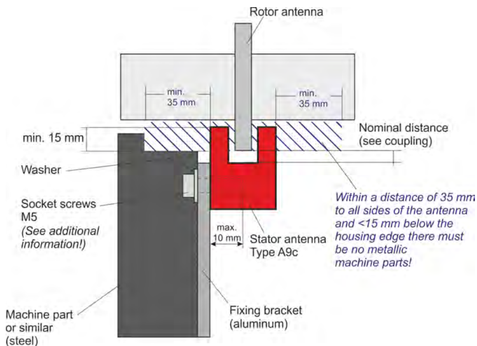
Fig. 6: Minimum distance antenna A9c
