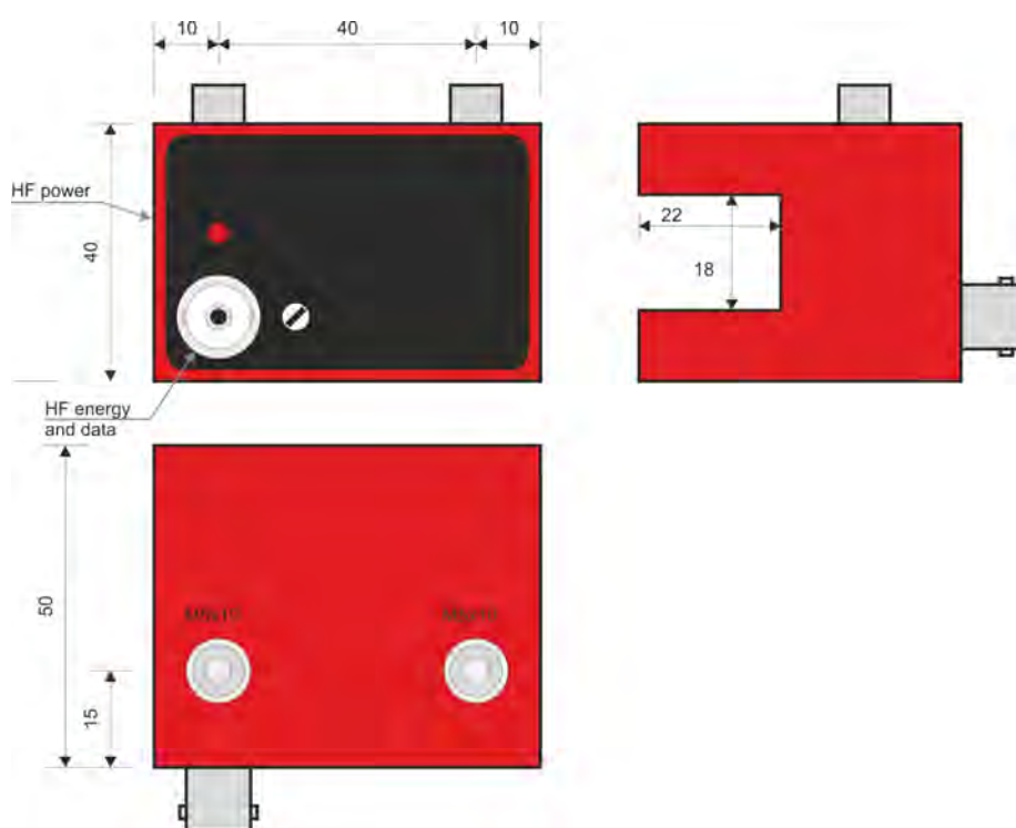
Fig. 4: Stator antenna A9c_PCM
