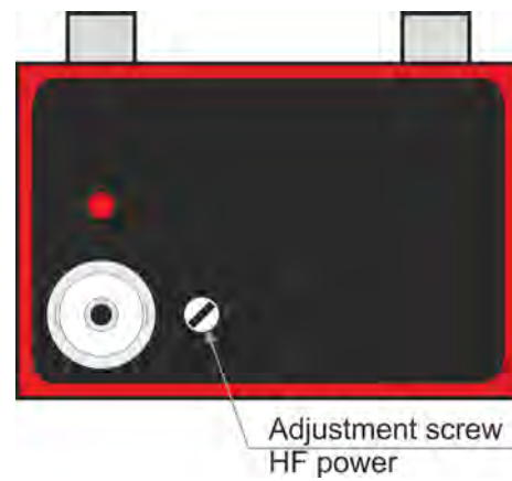
Fig. 7: Adjustment of stator antenna
