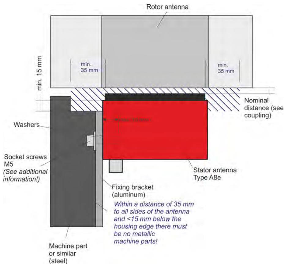
Fig. 6: Minimum distance antenna A8e
