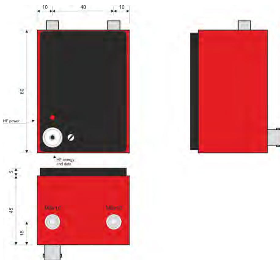
Fig. 4: Stator antenna A8e_PCM
