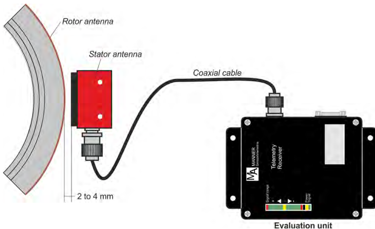
Fig. 8: Coupling
