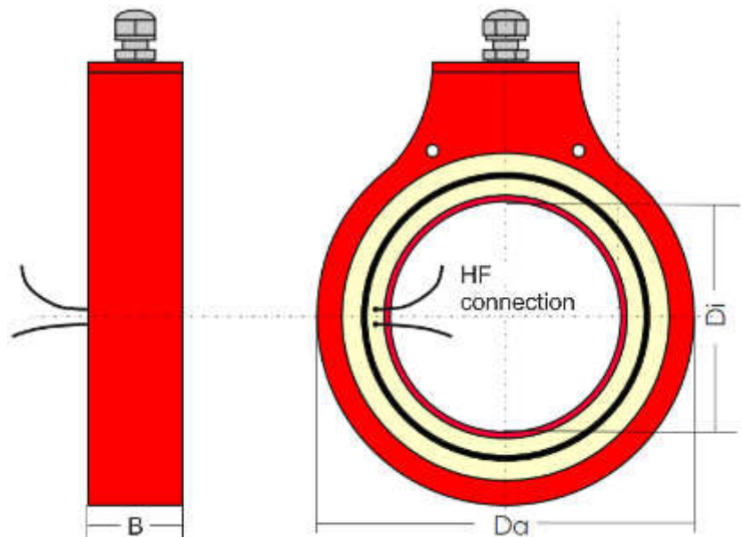
Fig. 5: Stator antenna A7_Lager_PCM
