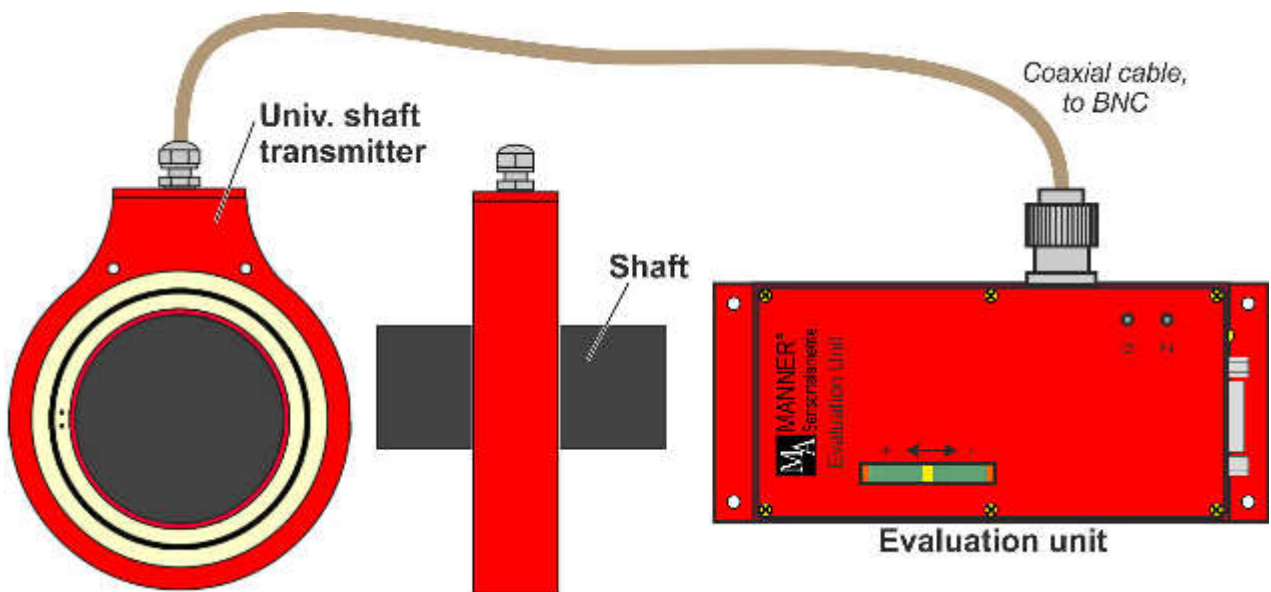
Fig. 6: Coupling
