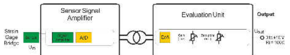
Fig. 2: Block diagram
