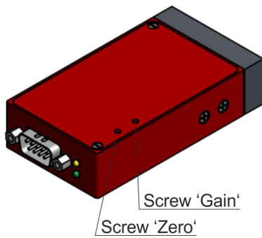
Fig. 6: Fine adjustment zeropoint and gain
