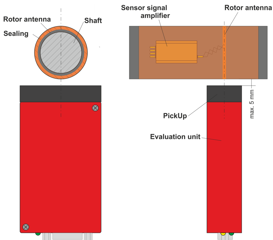
Fig. 5: Coupling
