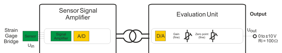
Fig. 2: Block diagram
