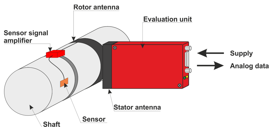
Fig. 1: General measuring configuration
