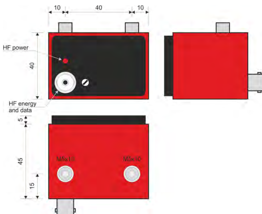
Fig. 4: Stator antenna A8c_PCM
