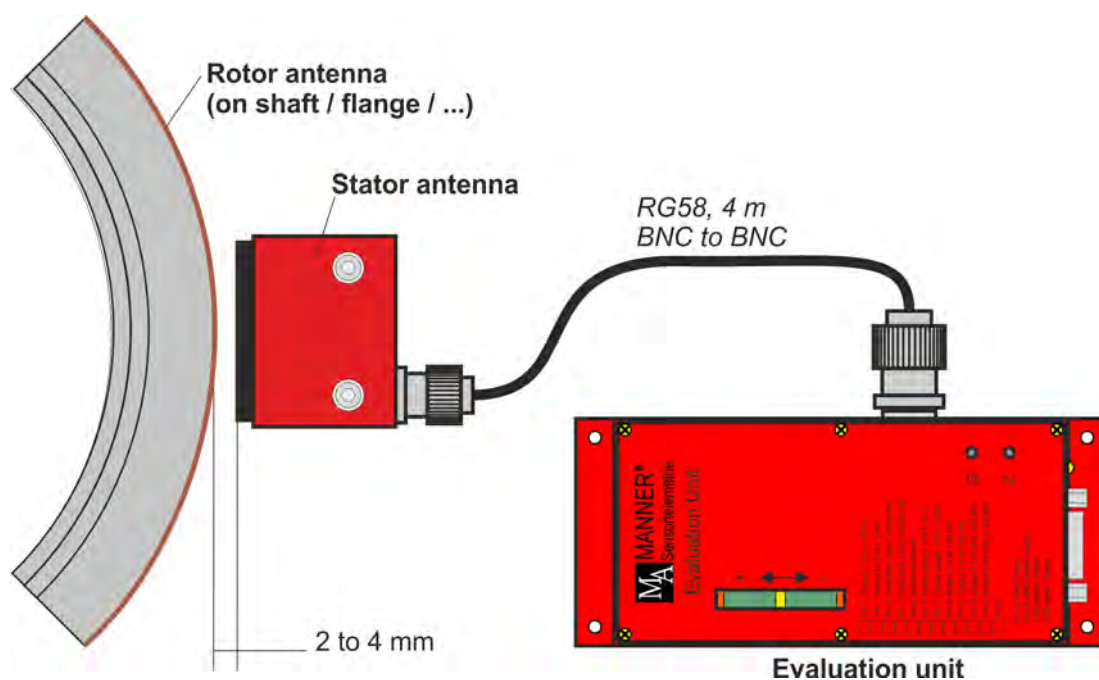
Fig. 5: Coupling
