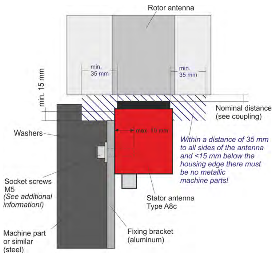
Fig. 6: Minimum distance antenna A8c
